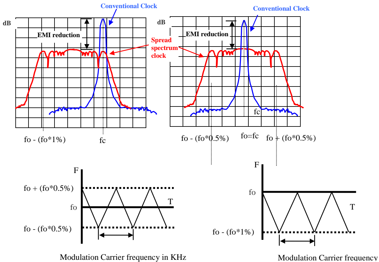
Figure 1: Spectrum comparisons of a -1% down spread and a \pm 0.5\% center spread
